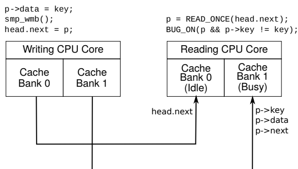
Figure 15.13: Why smp_read_barrier_depends() is Required
