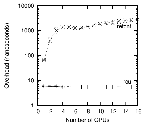
Figure 9.21: Performance of RCU vs. Reference Counting
