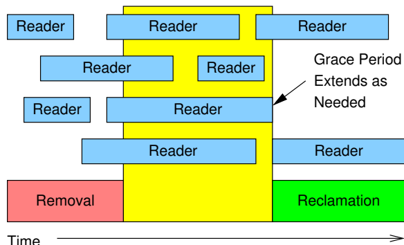
Figure 9.12: Readers and RCU Grace Period
