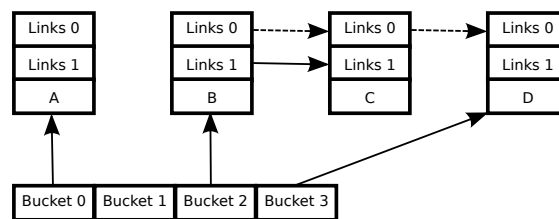
Figure 10.16: Growing a Double-List Hash Table, State (d)
