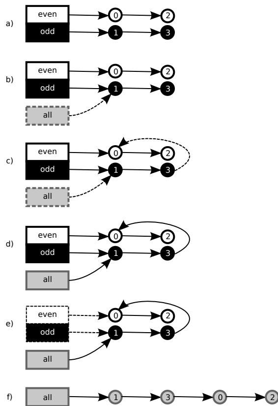
Figure 10.18: Shrinking a Relativistic Hash Table
