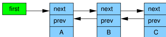
Figure 9.11: Linux Linear Linked List
