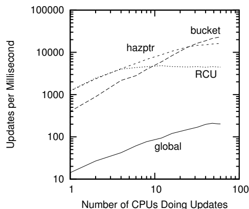
Figure 10.10: Update-Side RCU-Protected Hash-Table Performance For Schrödinger's Zoo at 60 CPUs
