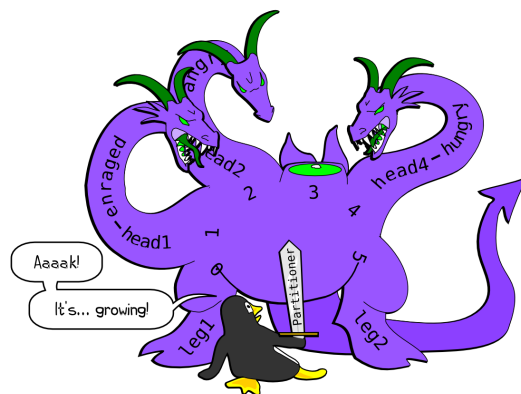
Figure 10.12: Partitioning Problems
