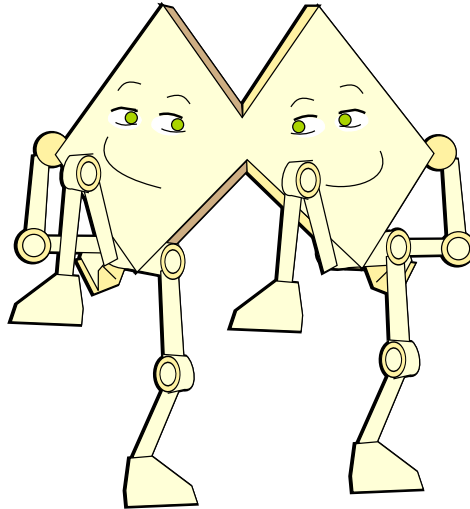
Figure 17.2: Multithreaded Mania
