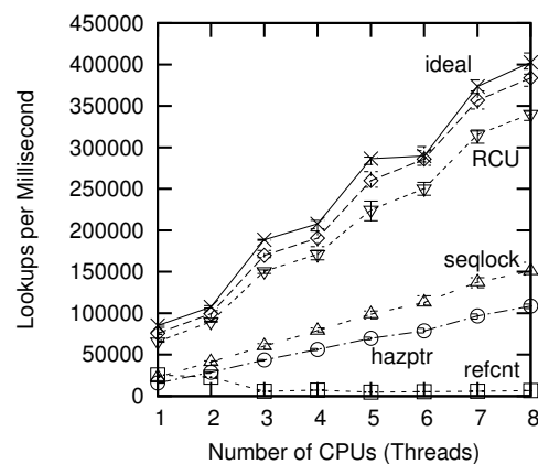
Figure 9.16: Pre-BSD Routing Table Protected by RCU QSBR
