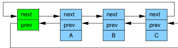
Figure 9.9: Linux Circular Linked List
