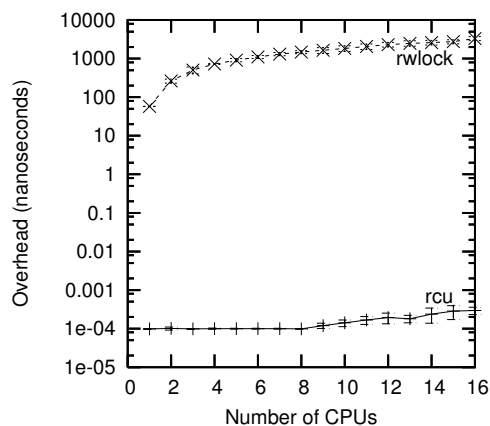
Figure 9.17: Performance Advantage of RCU Over Reader-Writer Locking
