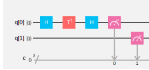
Figure 17.14: QC Program as Quantum Experience Score
