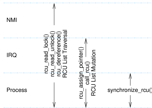
Figure 9.24: RCU API Usage Constraints
