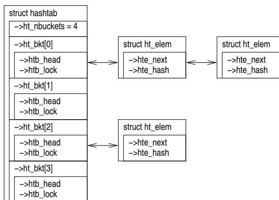
Figure 10.1: Hash-Table Data-Structure Diagram
