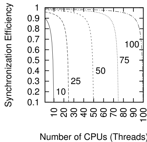
Figure 6.16: Synchronization Efficiency
