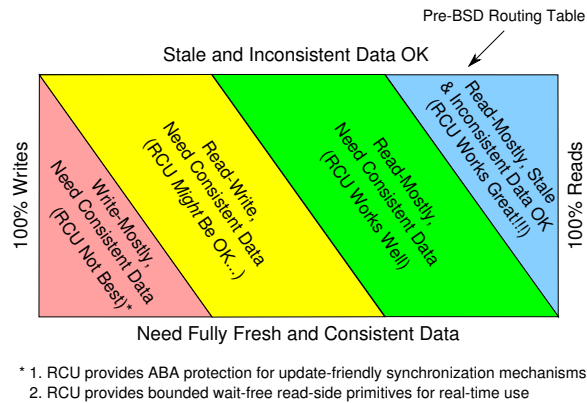
Figure 9.23: RCU Areas of Applicability
