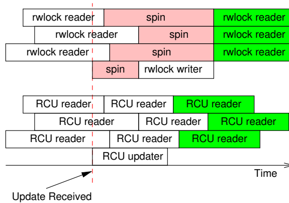
Figure 9.20: Response Time of RCU vs. Reader-Writer Locking
