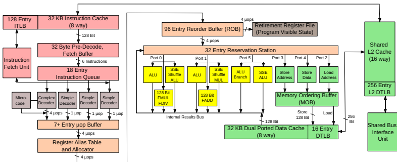
Figure 15.1: Intel Core 2 Architecture
