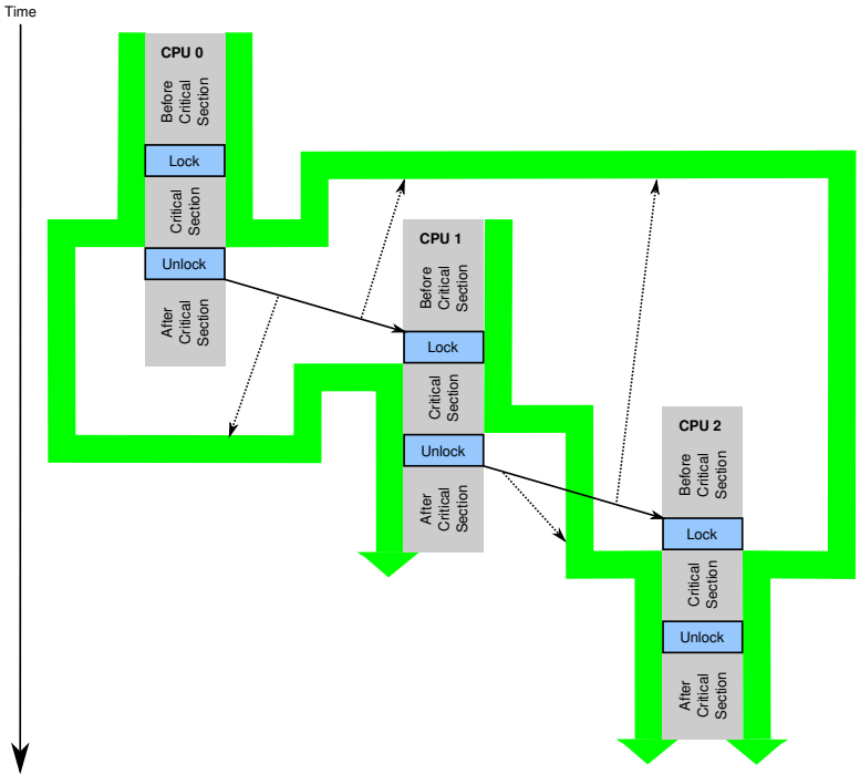
Figure 15.24: Locking Intuitions
