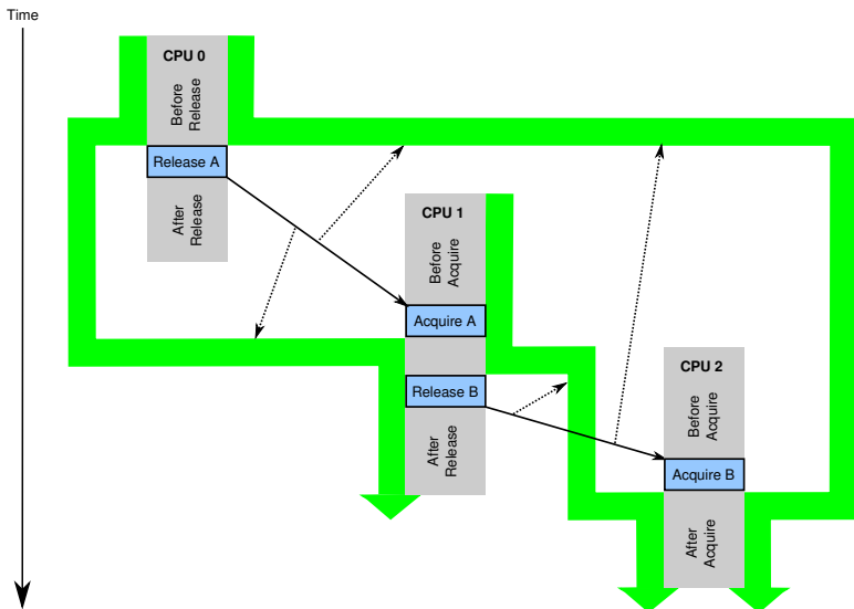
Figure 15.25: Release-Acquire Intuitions
