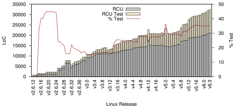
Figure 12.4: Linux-Kernel RCU Test Code
