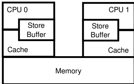
Figure 15.3: System Architecture With Store Buffers
