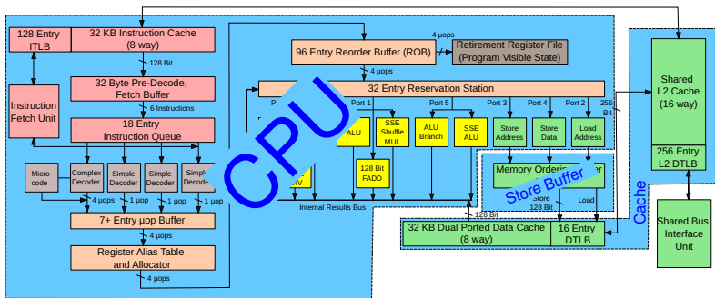
Figure 15.2: Intel Core 2 Architecture Simplified
