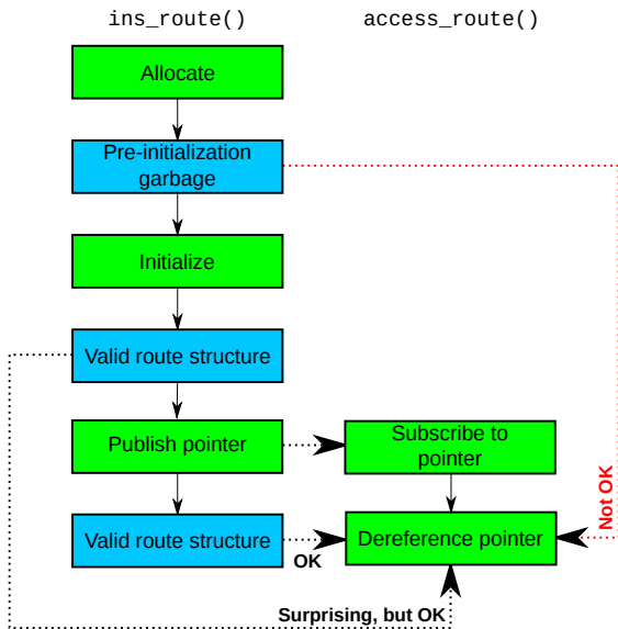
Figure 9.10: Publication/Subscription Constraints
