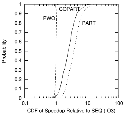
Figure 6.30: Partitioned Coroutines
