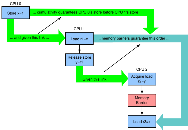
Figure 15.11: Cumulativity
