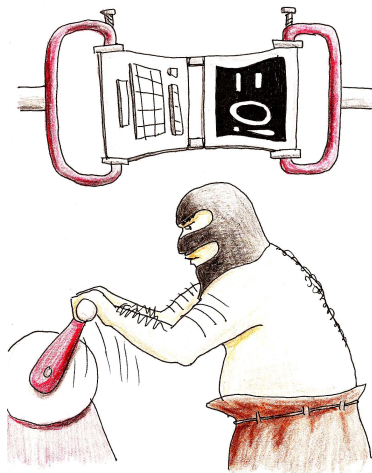
Figure 11.2: Rationalizing Validation
