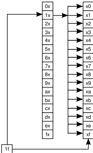
Figure 14.9: Timer Wheel
