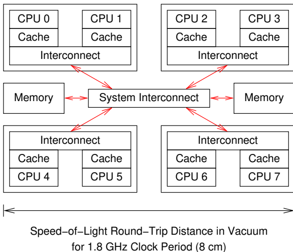
Figure 3.11: System Hardware Architecture
