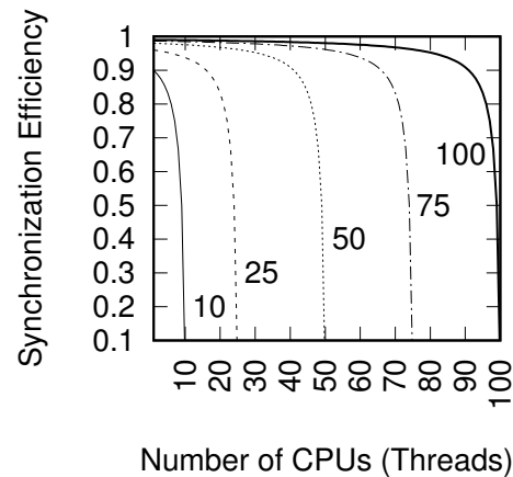
Figure 6.16: Synchronization Efficiency
