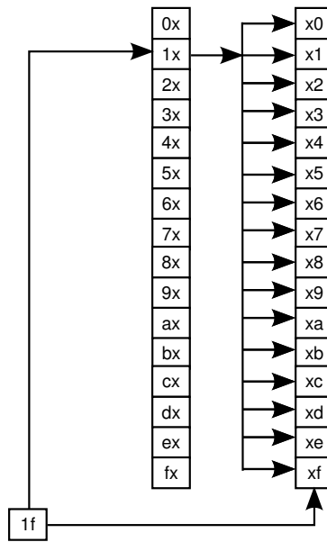
Figure 14.9: Timer Wheel
