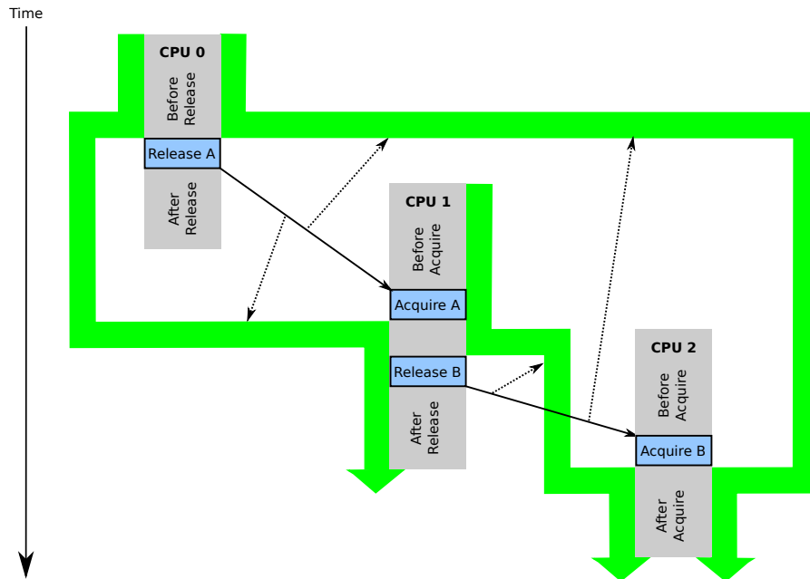
Figure 15.2: Release-Acquire Intuitions
