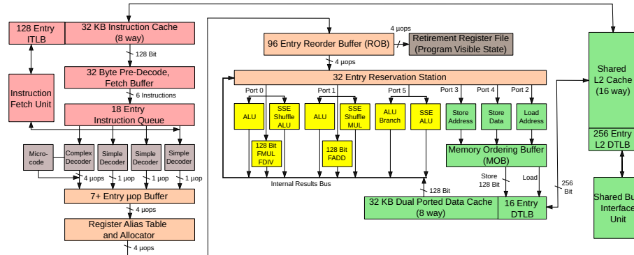
Figure 15.4: Intel Core 2 Architecture
