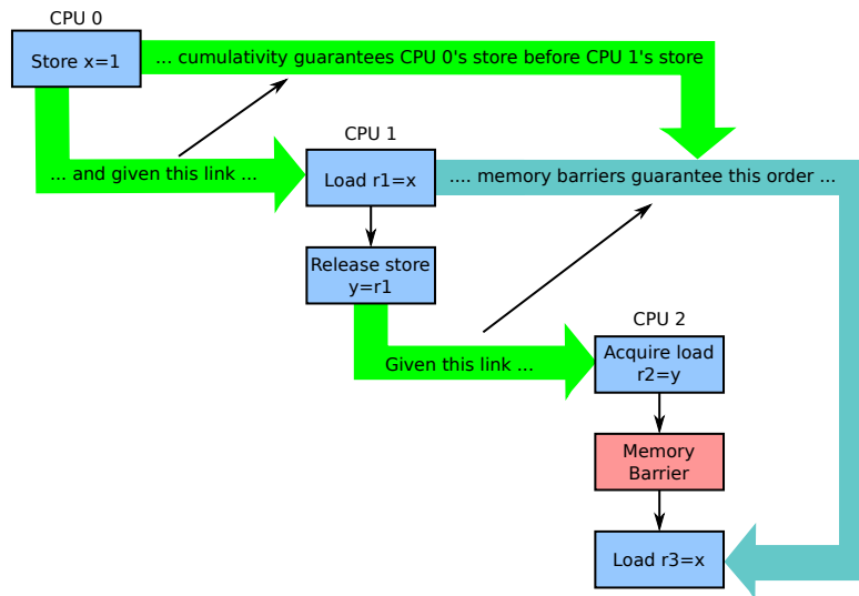
Figure 15.14: Cumulativeness
