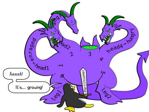
Figure 10.13: Partitioning Problems
